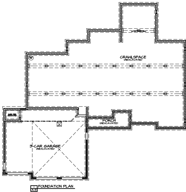
FOUNDATION PLAN A-2
