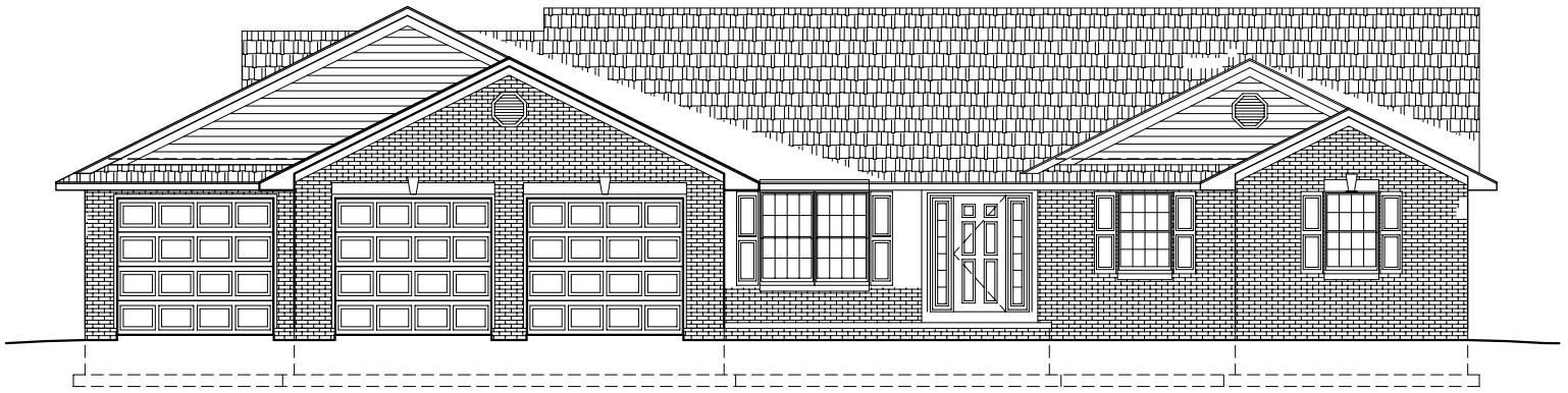
FRONT ELEVATION A-1
