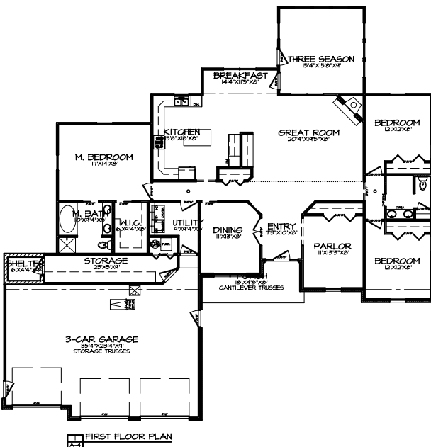
FIRST FLOOR PLAN A-3
